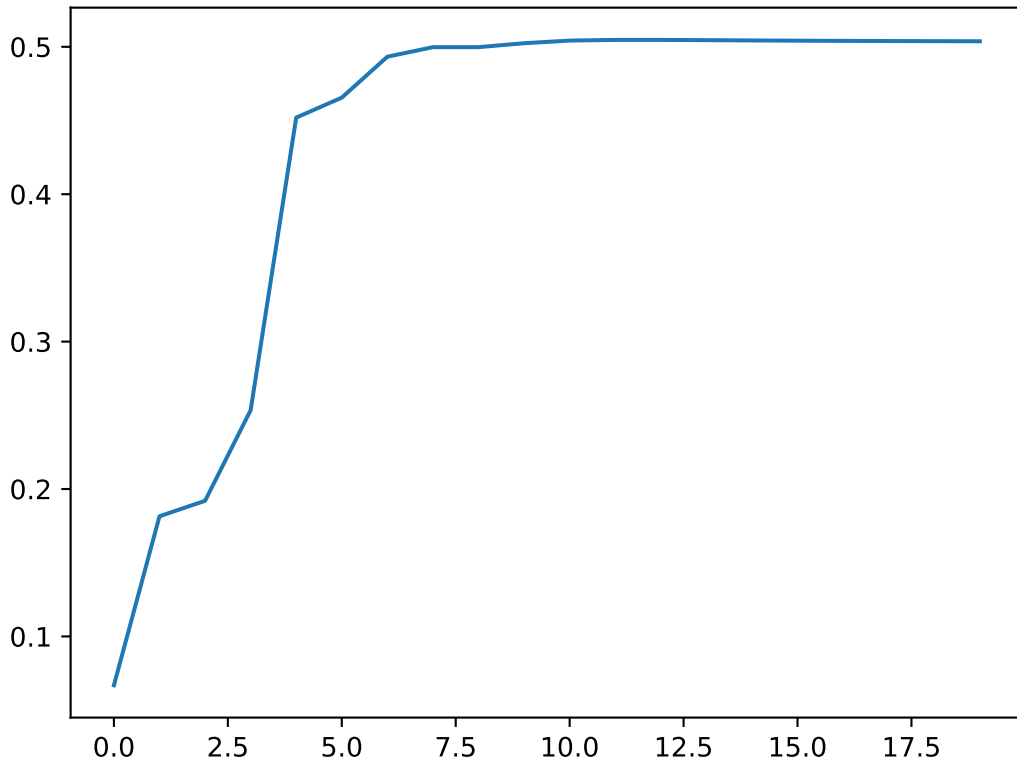
Strehl ratio
