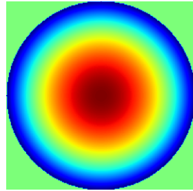
4 Z_2^0 defocus
